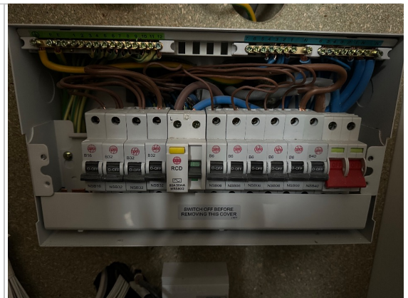
Image of layout of consumer unit
