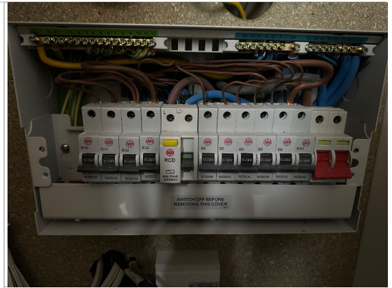
Internals of consumer unit
